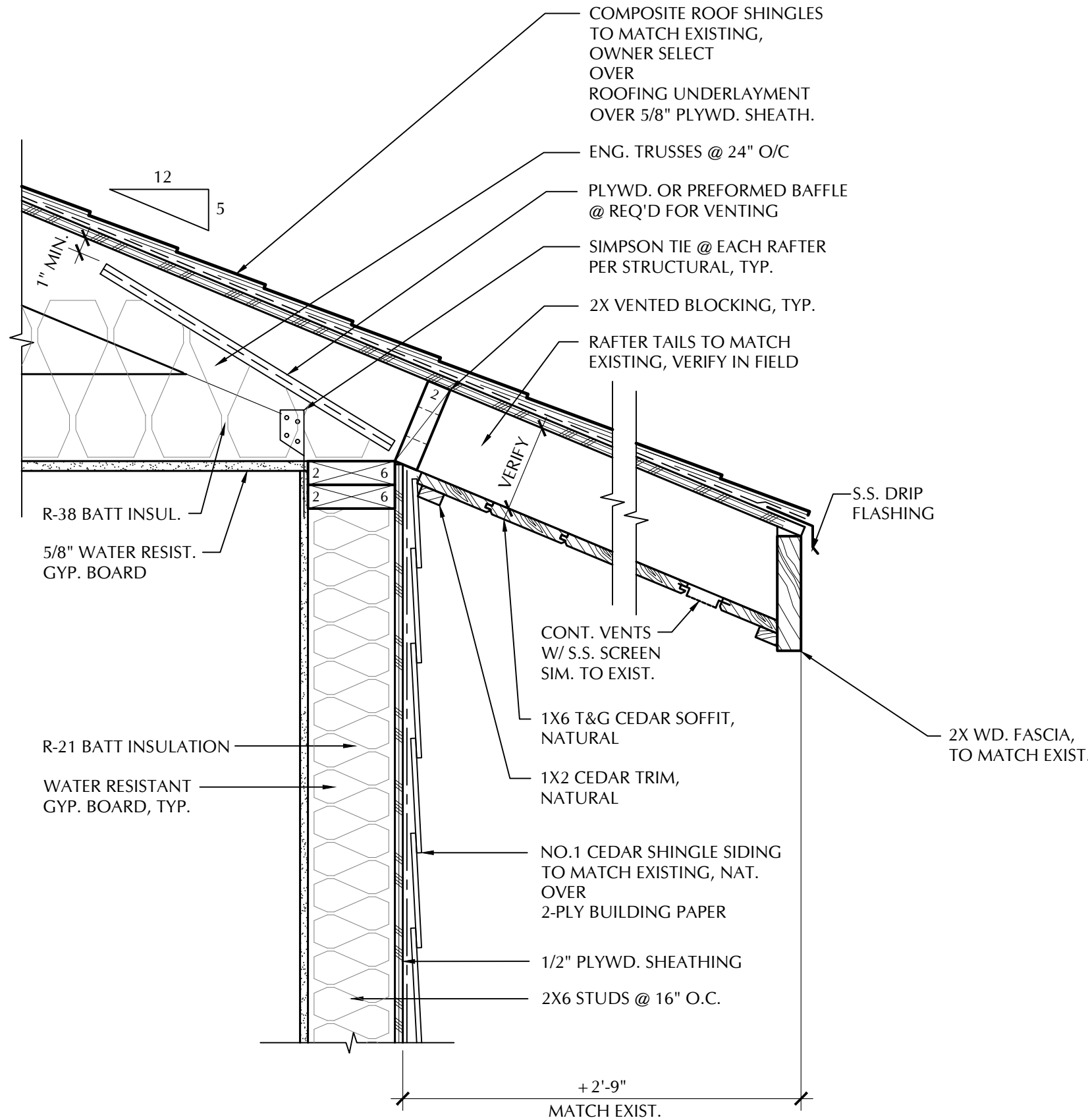
5 A2.1 1 1/2" = 1'-0"
