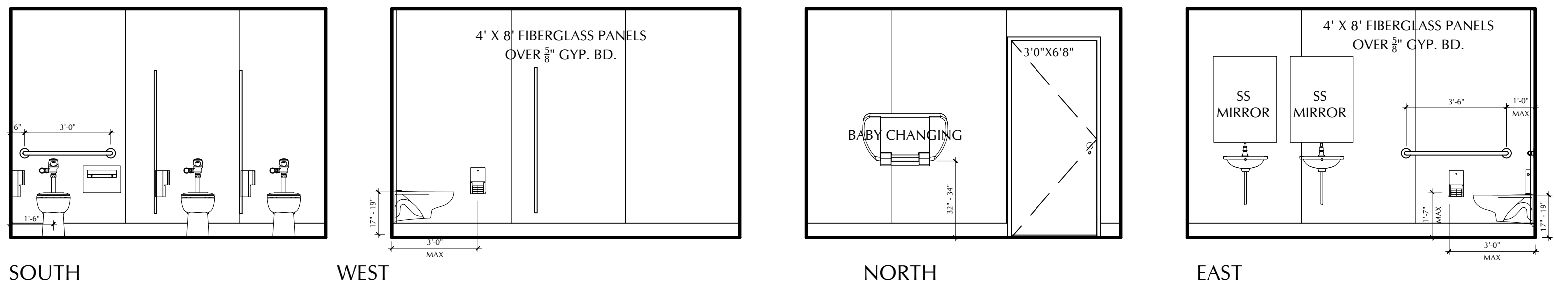
4 NEW WOMENS RESTROOM ELEVATIONS A1.2 3/8" = 1'-0"
