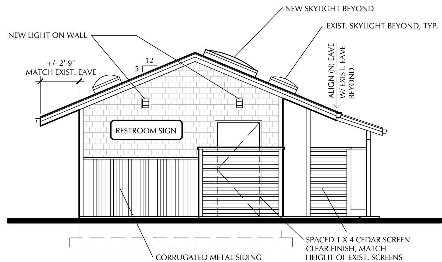
3 A2.1 1/4" = 1'-0"
