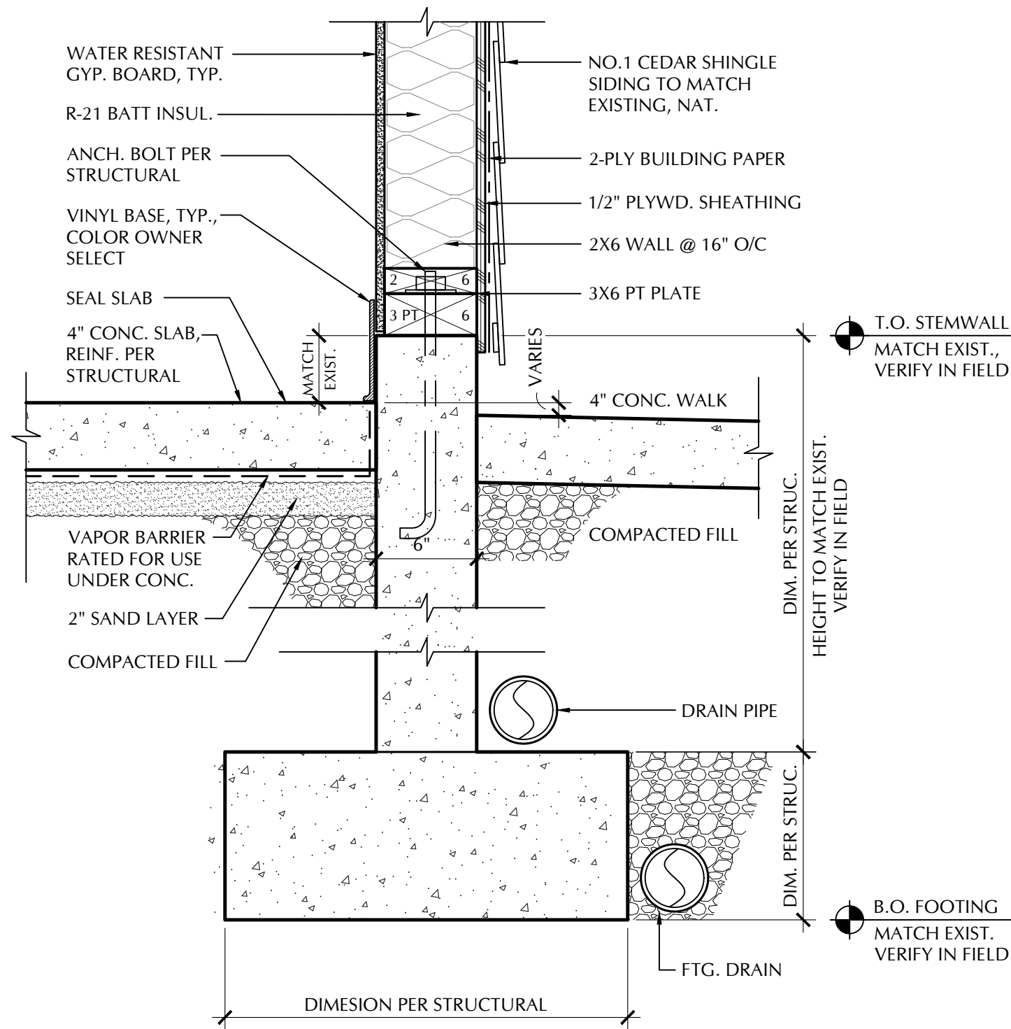
2 TYP. STEMWALL S1.1 1 1/2" = 1'-0"
