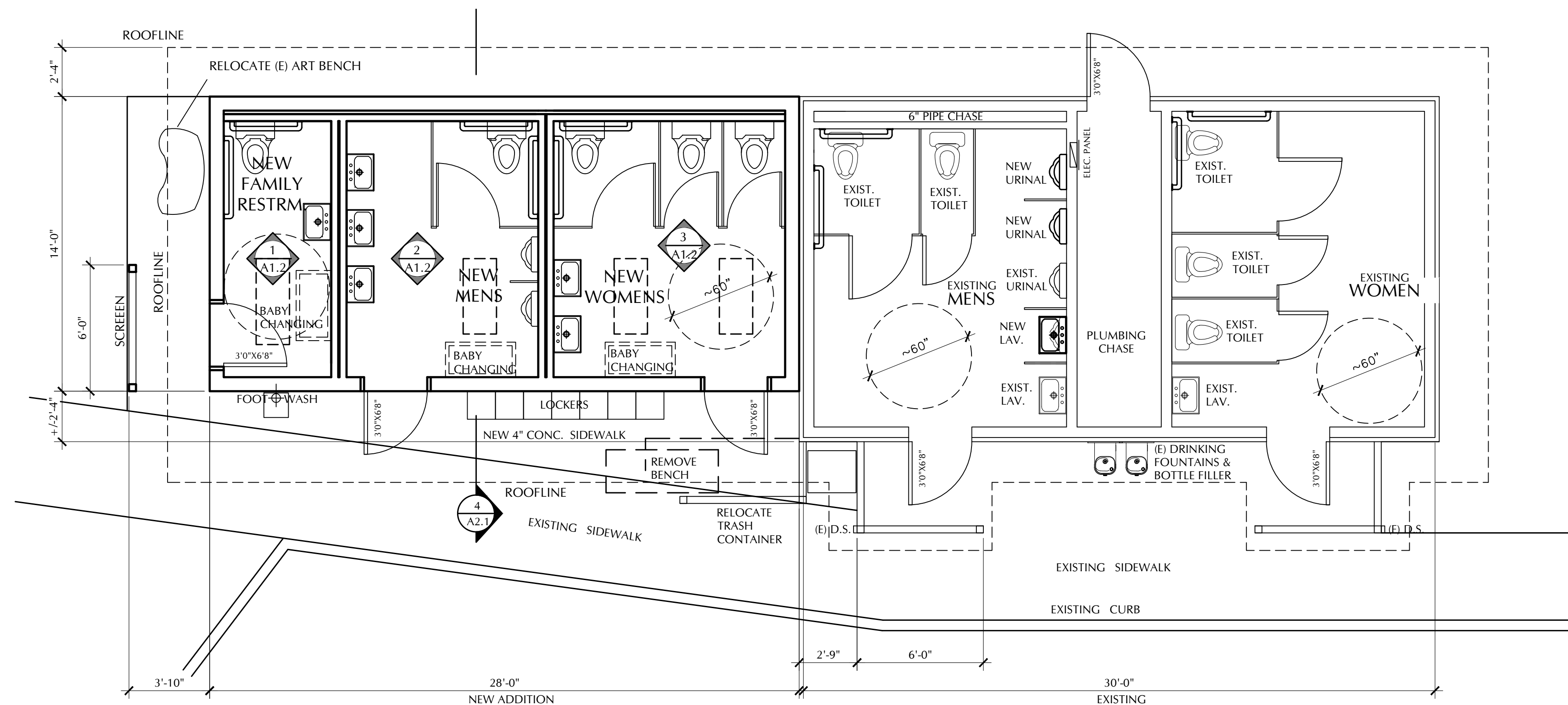
1 MIDTOWN RESTROOM ADDITION A1.1 1/4" = 1'-0"
