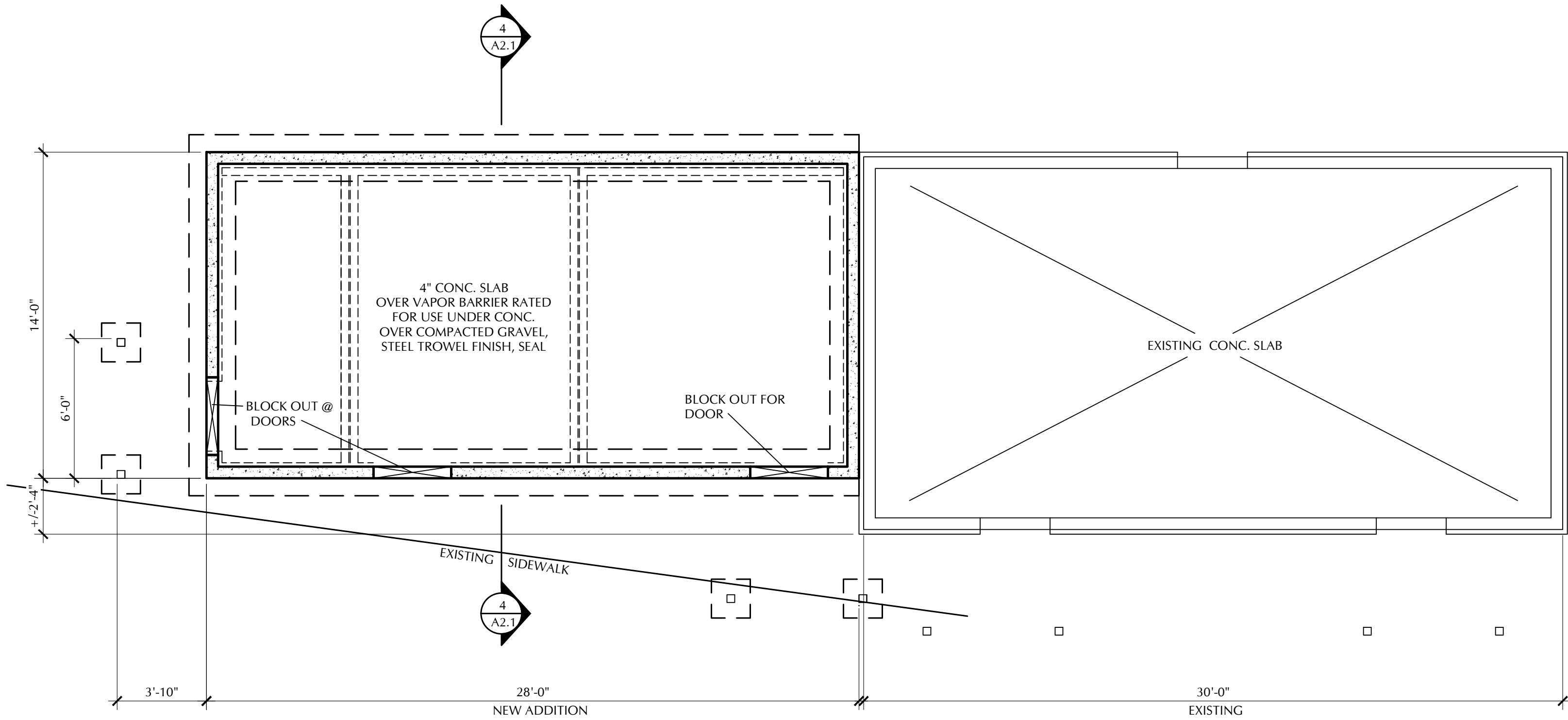
1 MIDTOWN RESTROOM FOUNDATION PLAN S1.1 1/4" = 1'-0"
