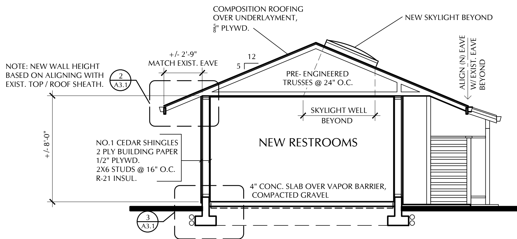
4 A2.1 1/4" = 1'-0"
