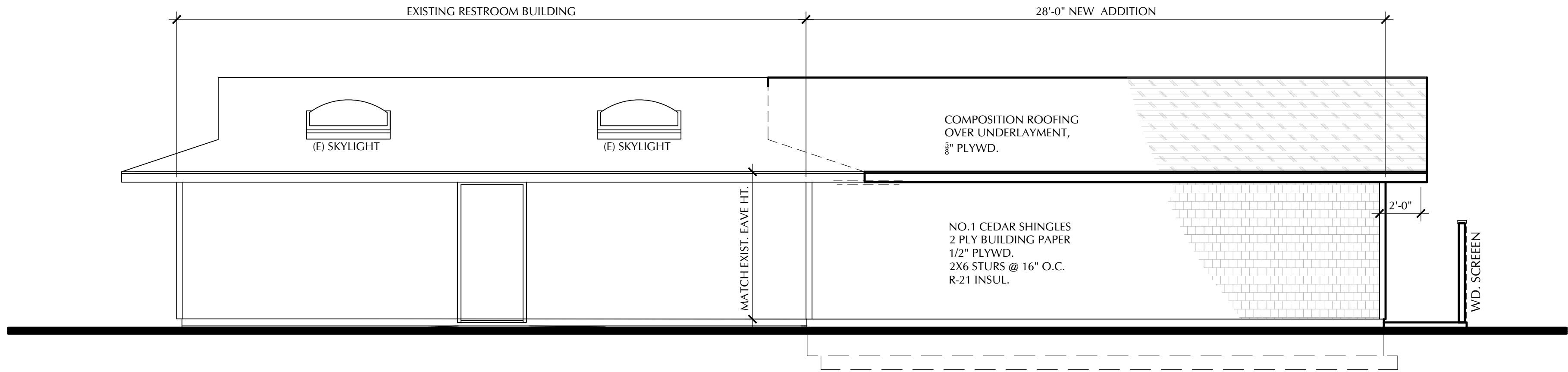
2 A2.1 1/4" = 1'-0"
