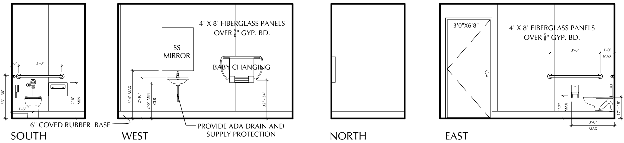
FAMILY RESTROOM ELEVATIONS
