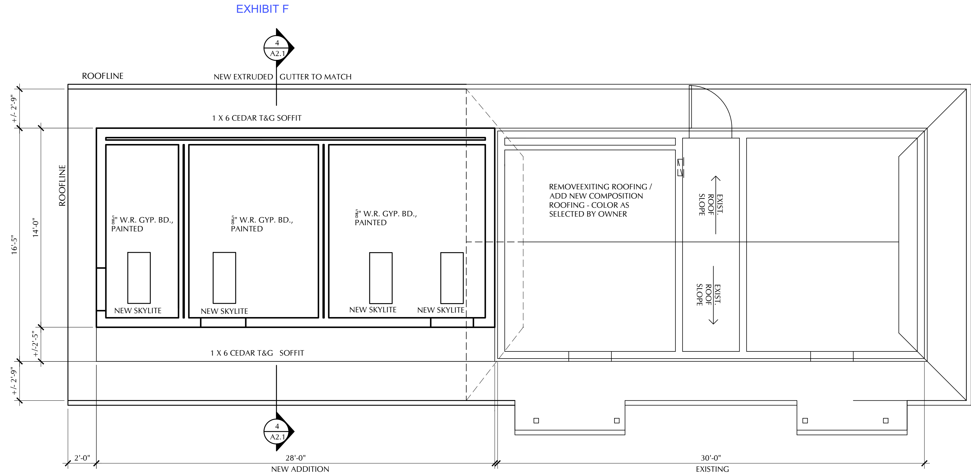
1 MIDTOWN RESTROOM CEILING PLAN
